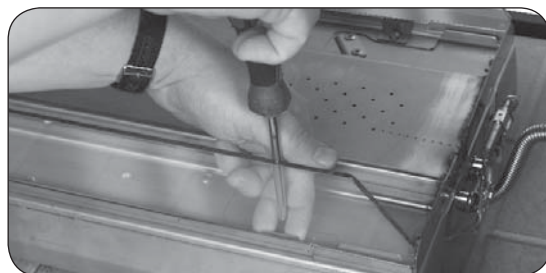
Fig. 15-5 Securing Glass Panel
